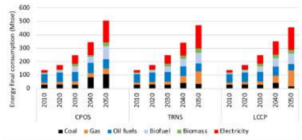
Figure 14. Projection of final energy demand by fuel type under CPOS, TRNS and LCCP
