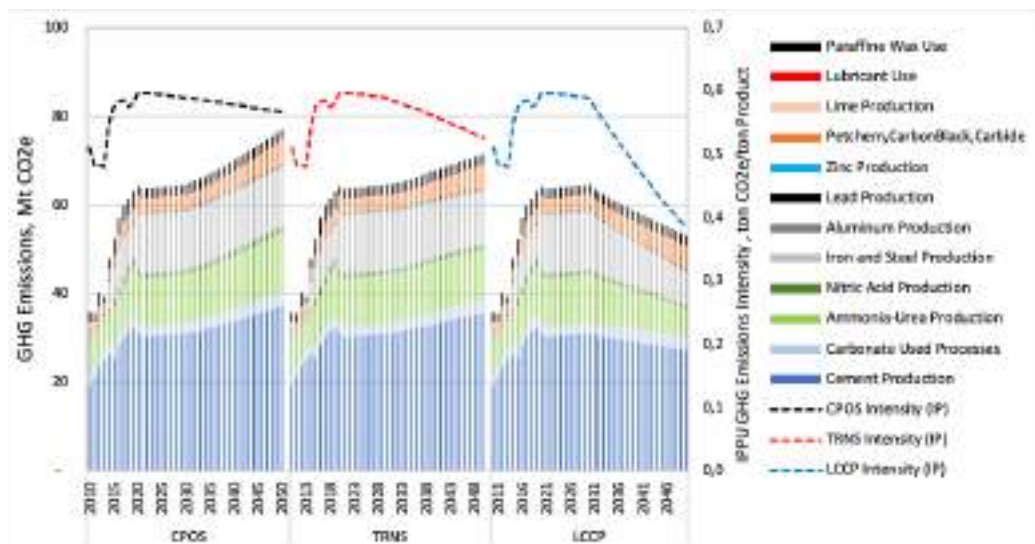
Figure 30. IPPU GHG emissions development and projections of CPOS, TRNS and LCCP
