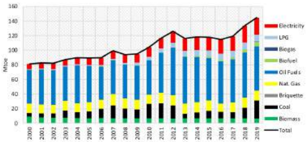
Figure 10. Development of final energy consumption by type of fuels
