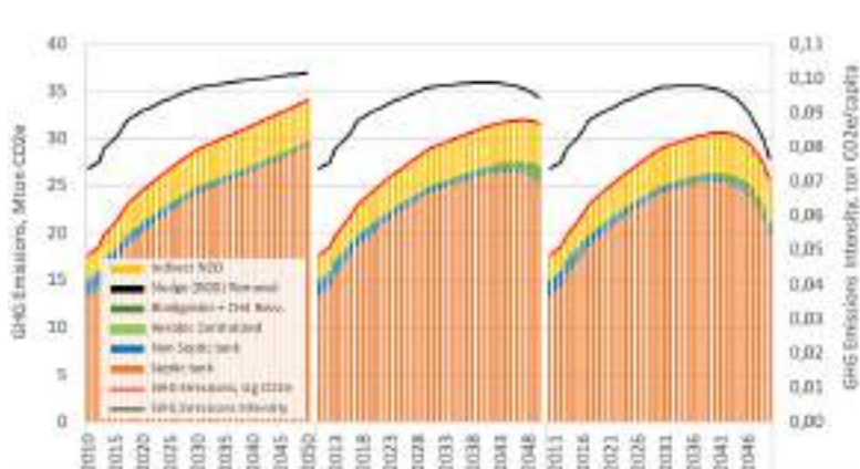
Figure 27. The projection of GHG emissions level and intensity of Domestic WWT
